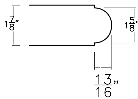
BULLNOSE DETAIL
