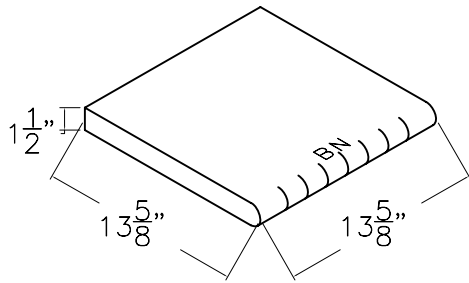
DC-1414 POOL COPING
