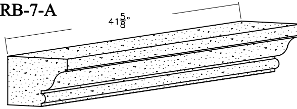
STRETCHER
